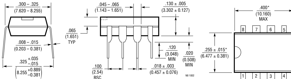
N Package 8-Lead PDIP (Narrow 0.300) (LTC DWG # 05-08-1510)
