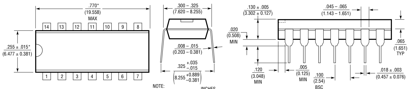
N Package 14-Lead PDIP (Narrow 0.300) (LTC DWG # 05-08-1510)
