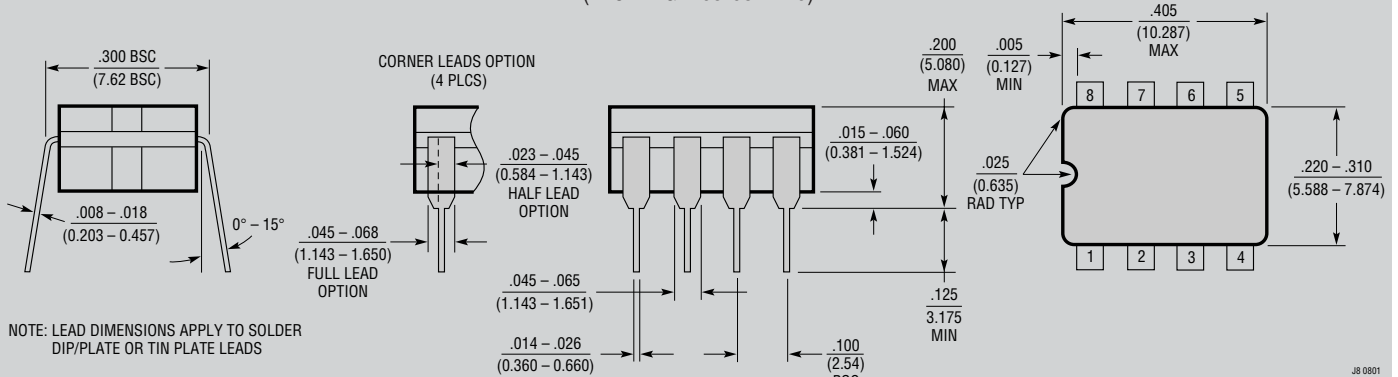
J Package 8-Lead CERDIP (Narrow 0.300, Hermetic) (LTC DWG # 05-08-1110)
